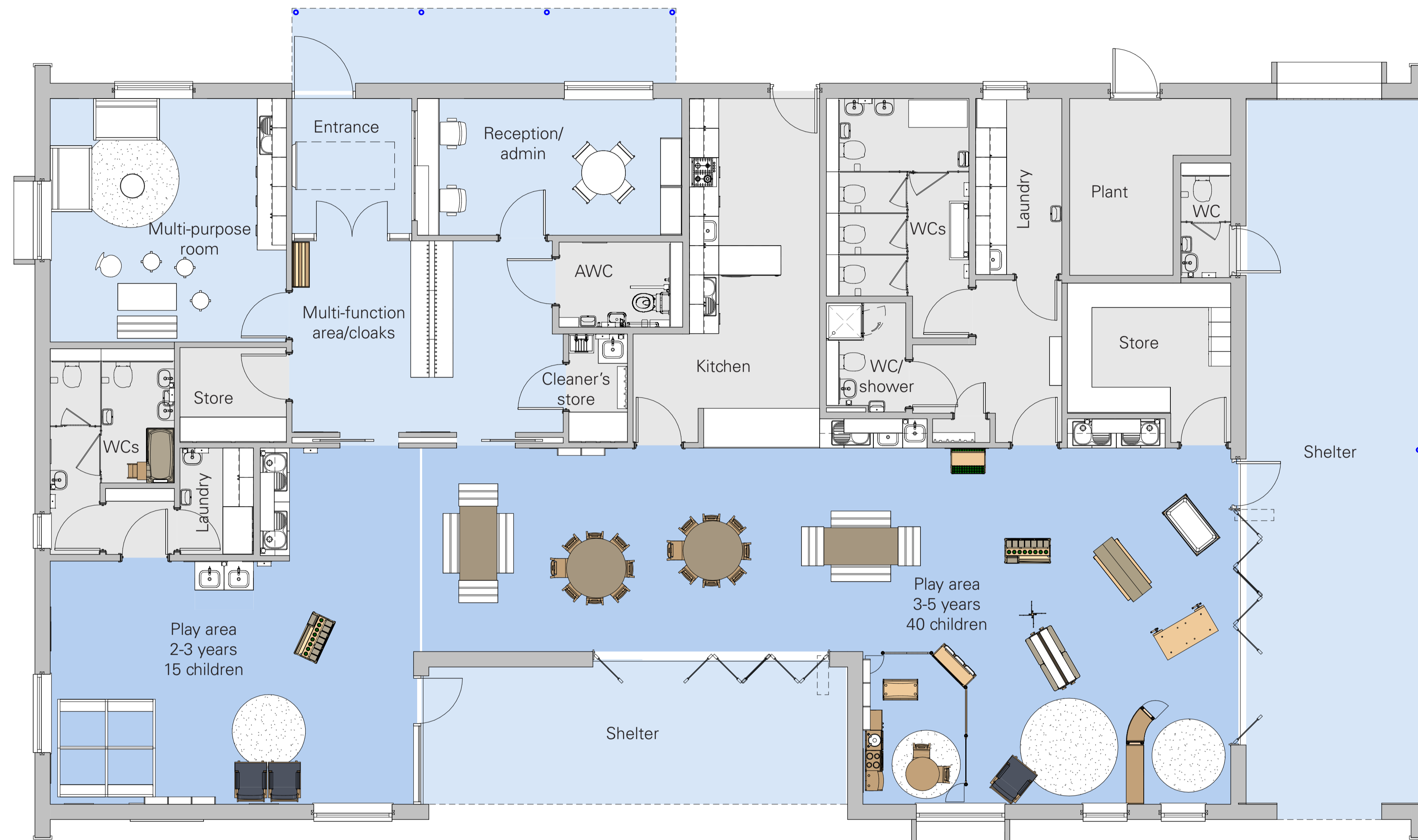
1 Playroom - ground floor plan
