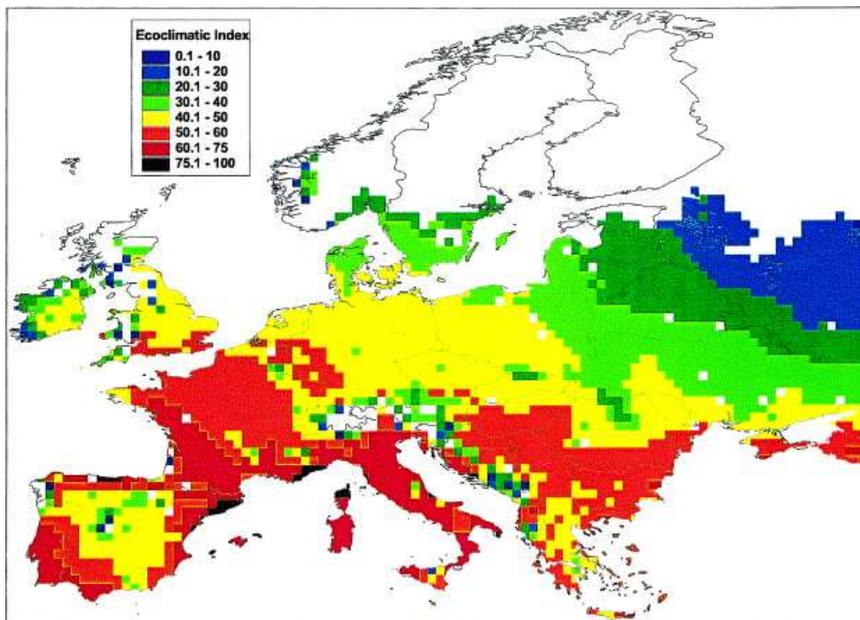
Figure 23. Ecoclimatic Indices for countries across Europe. An index of >32 is suggested to be suitable for ALB (Ref: MacLeod et al. , 2002).
