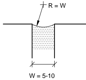
DETAIL OF POINTING
