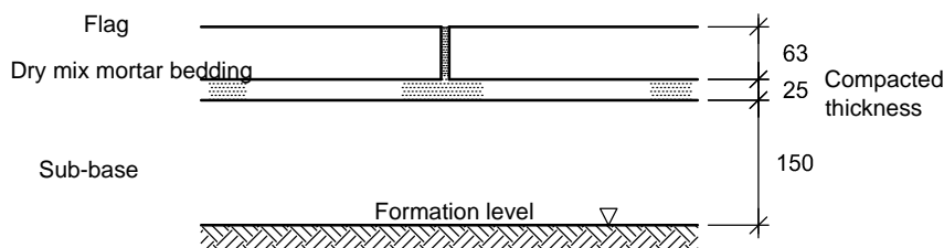
SECTIONAL ELEVATION
