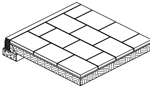
PAVING LAYOUT
