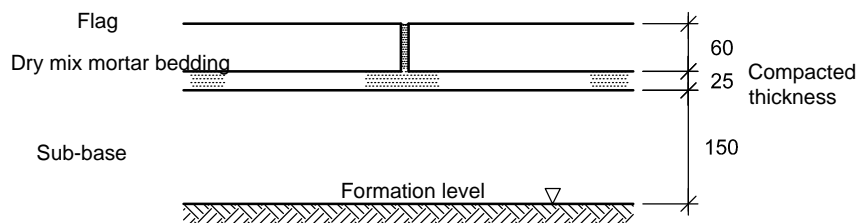
SECTIONAL ELEVATION
