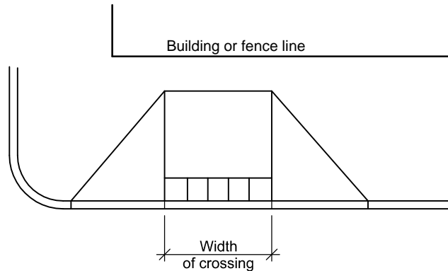
TYPICAL LAYOUT 1 AT INSET DROP KERB CROSSING
