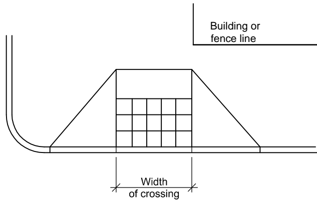
TYPICAL LAYOUT 2 AT IN-LINE DROP KERB CROSSING
