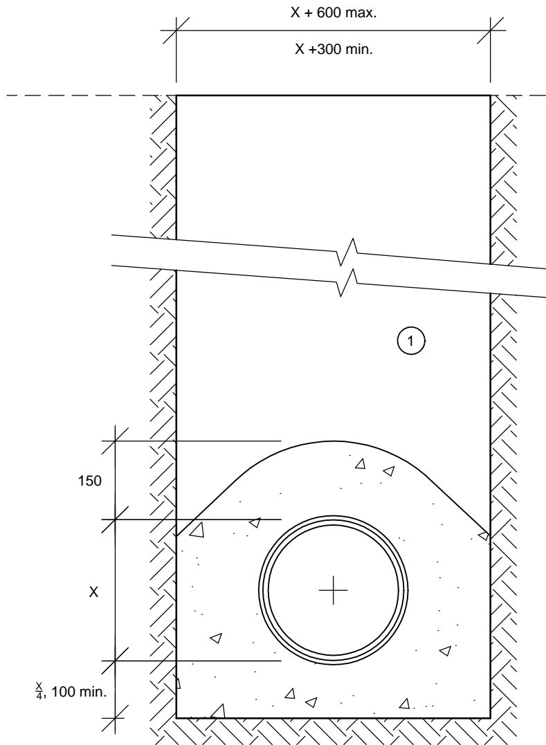
Bed Type Z CONCRETE SURROUND
