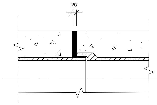
DETAIL OF EXPANSION JOINT FOR CONCRETE SURROUND
