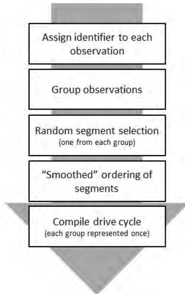
Figure 23: Drive cycle development process
