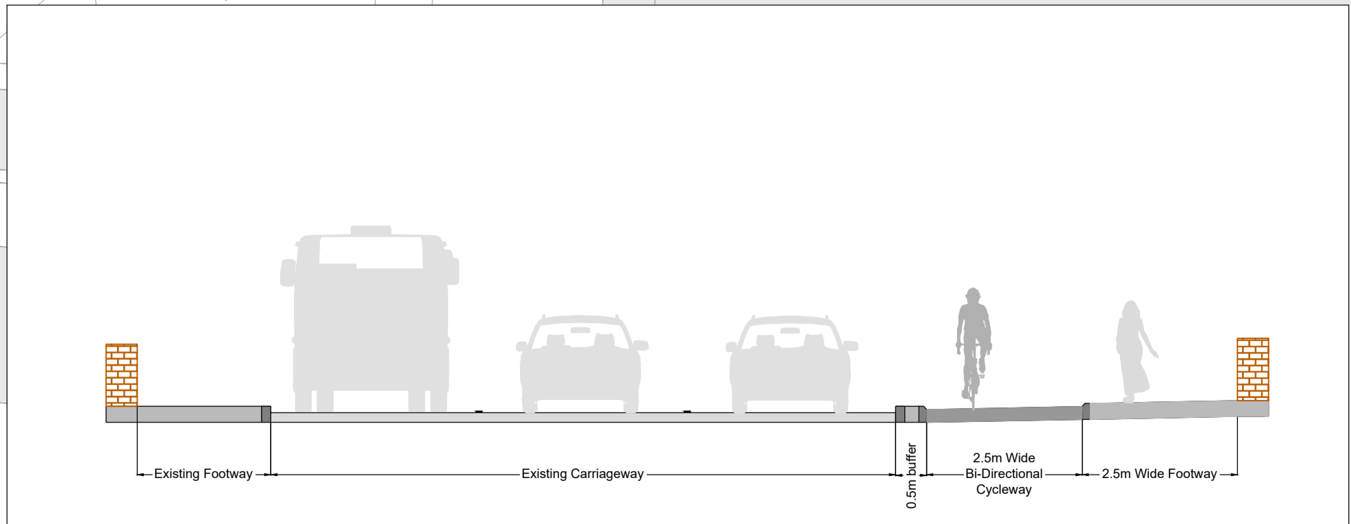
Section AA - Cross Section
